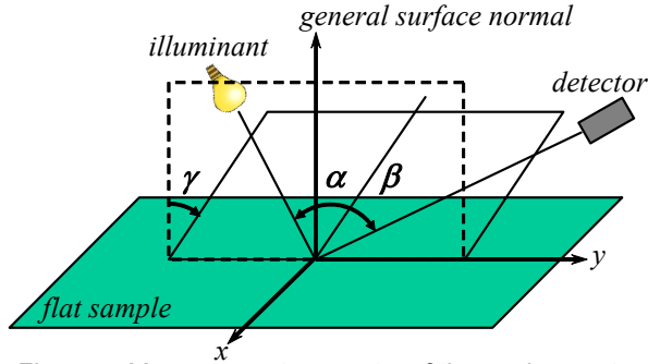
Figure 7. Measurement geometry of the gonio-spectro-photometric colorimeter GCMS-4
