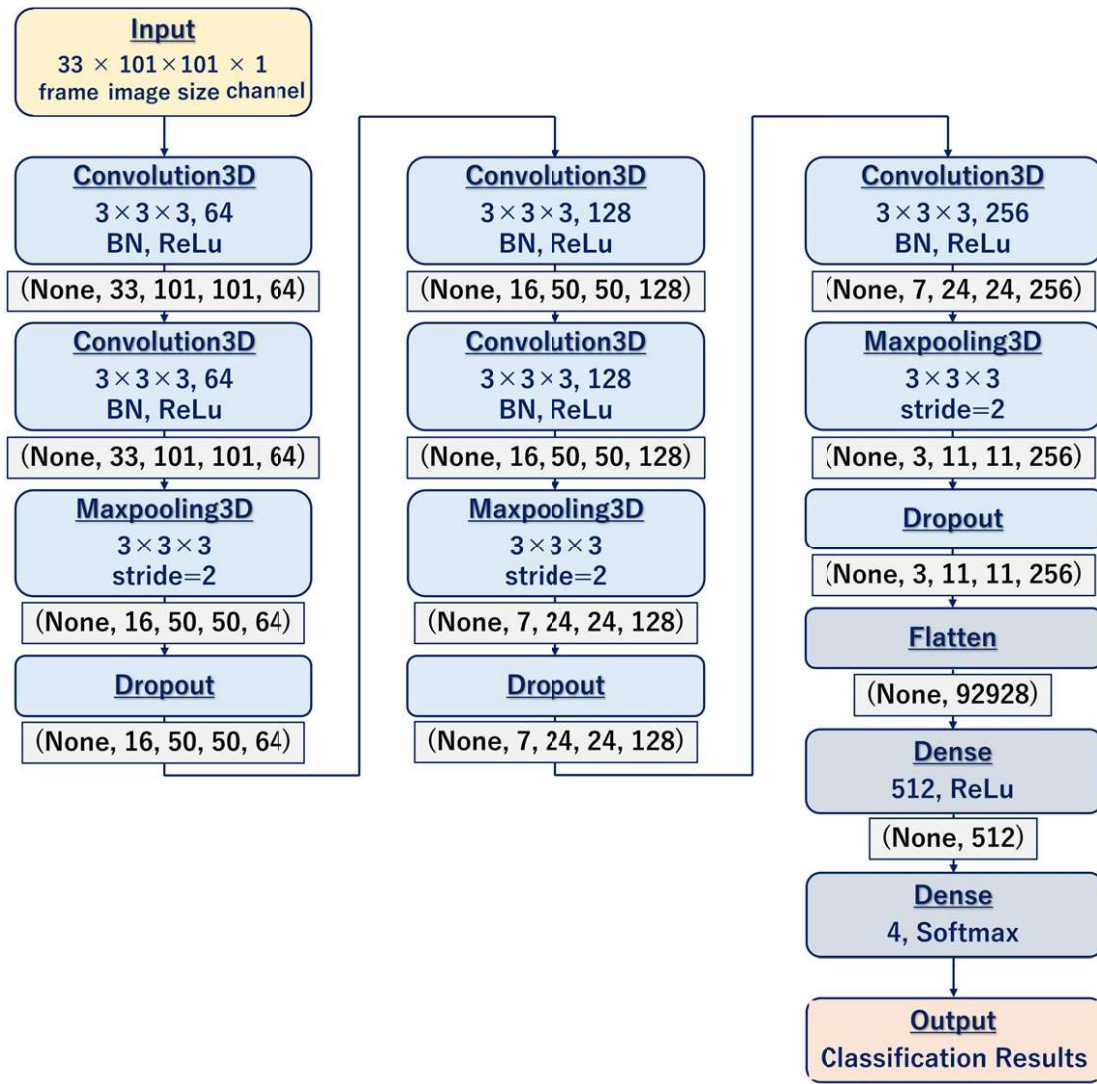
Figure 15. Network architecture.
