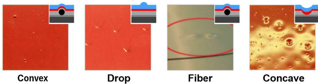
Figure 1. Schematic and image of paint defects.
